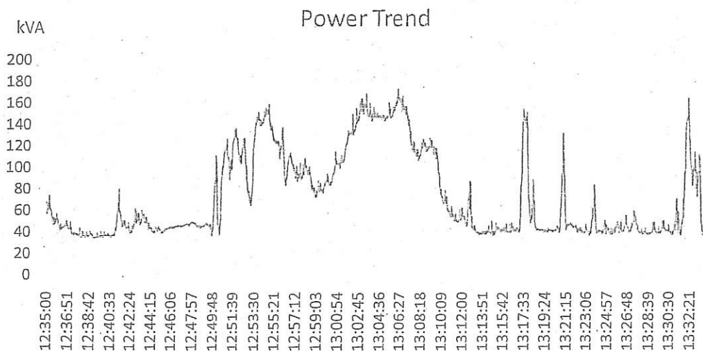
Figure 17- Engineering College Power Consumption Profile – kVA
