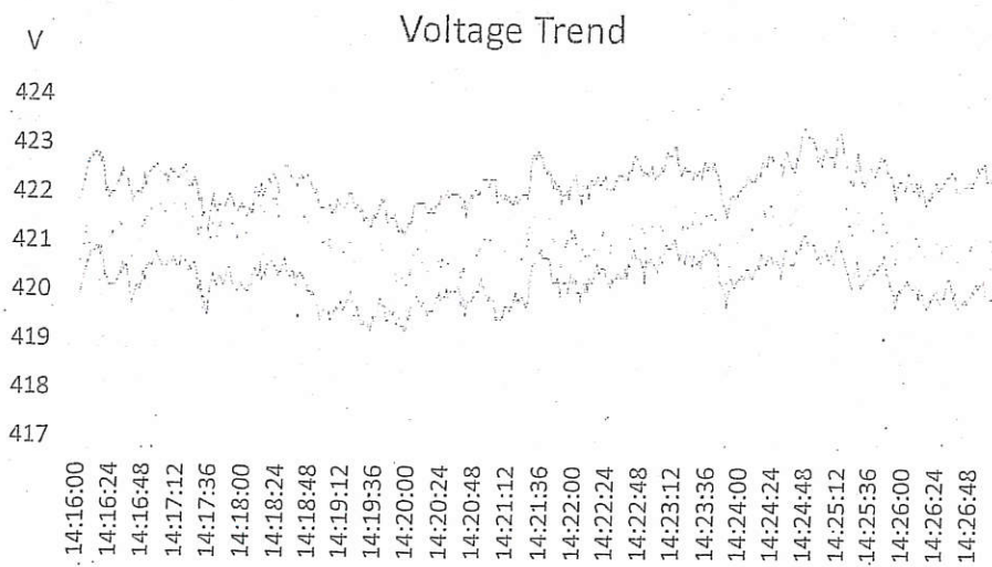
Figure 19-College of Management Voltage Profile
