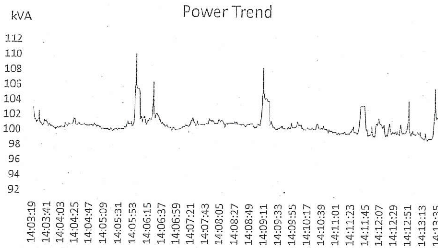
Figure 27-College of Pharmacy Power Consumption Profile – kVA
