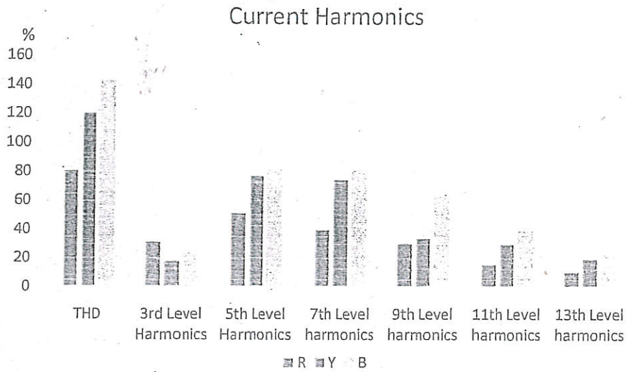
Figure 10- Current Harmonics-Engineering College
