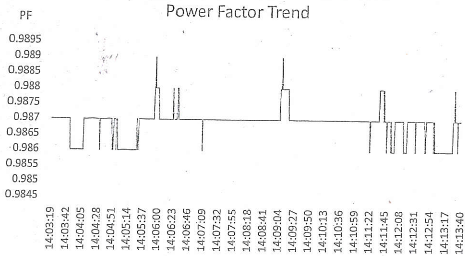
Figure 28- College of Pharmacy Power Factor Profile
