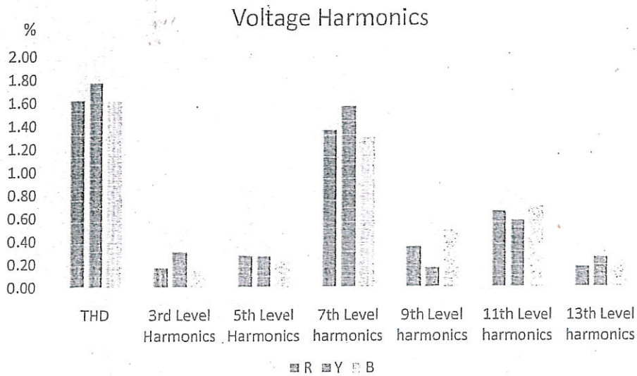
Figure 8-. Voltage Harmonics Profile – College of Pharmacy
