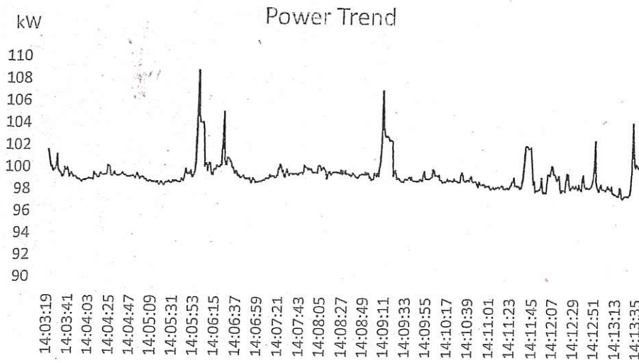
Figure 26- College of Pharmacy Power Consumption Profile – kW
