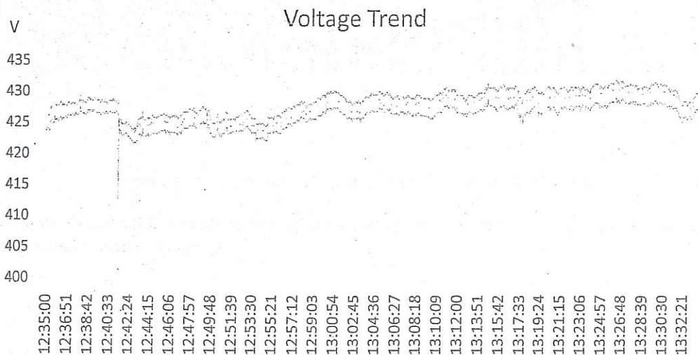
Figure 14- Engineering College Voltage Profile
