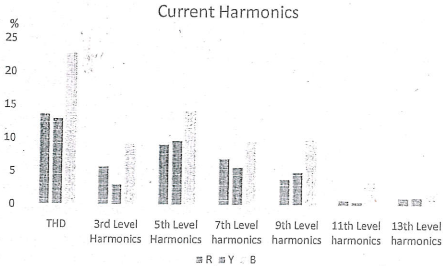
Figure 13- Current Harmonics – Polytechnic College
