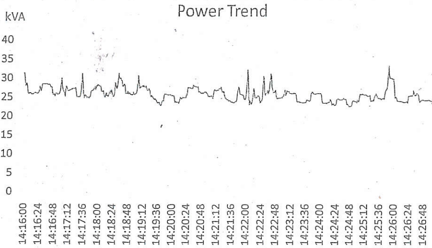
Figure 22-College of Management Power Consumption Profile – KVA
