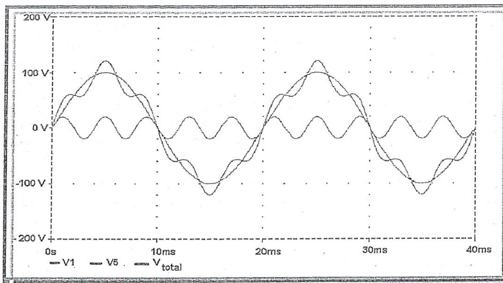
Figure 4- Harmonics
