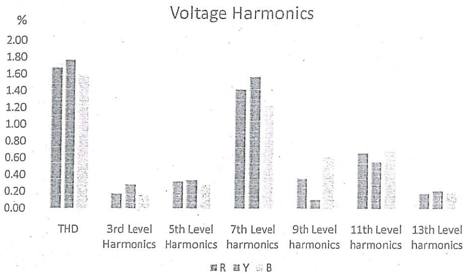
Figure7. Voltage Harmonics Profile – Management College
