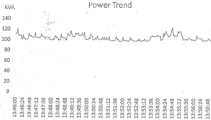
Figure 31-College of Polytechnic Power Consumption Profile – KVA
