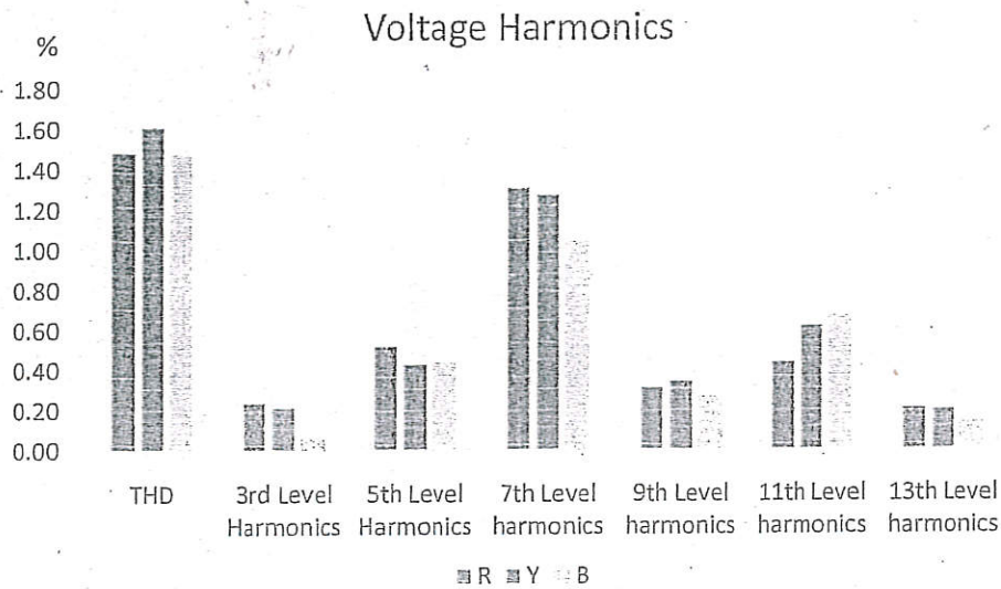
Figure 9- Voltage Harmonics Profile – Polytechnic College
